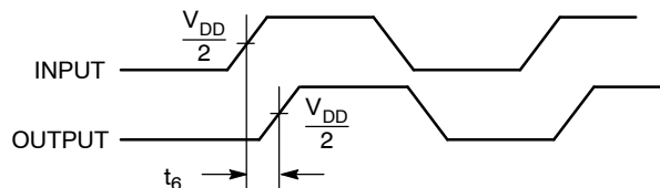
Figure 6. Input - Output Propagation Delay
