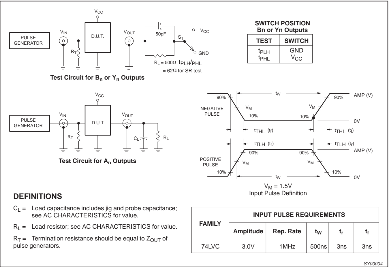
Waveform 5.
