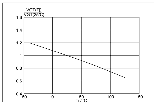
Fig.6. Normalised gate trigger voltage V_{GT}(T_j)/V_{GT}(25\text{ °C}) , versus junction temperature T_j .
