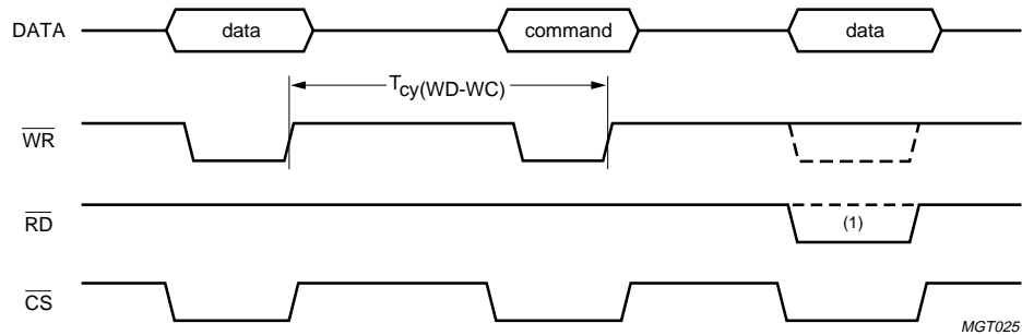
Fig 22. Write data + write command cycle timing.
