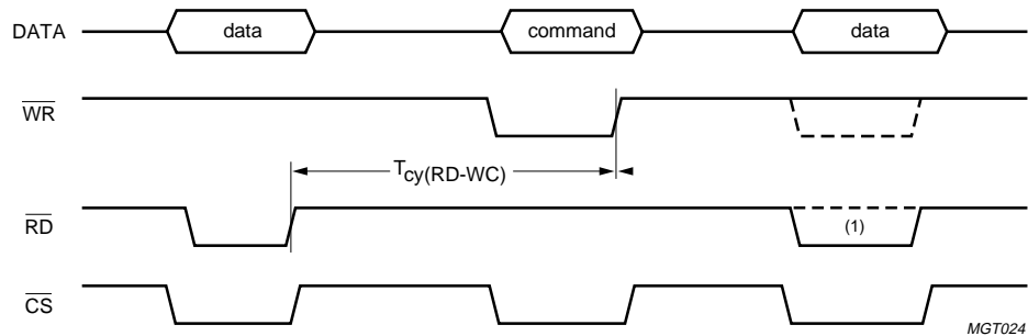
Fig 24. Read data + write command cycle timing.
