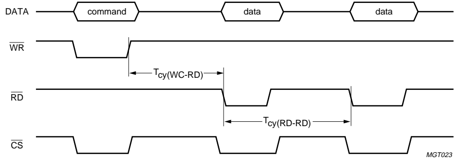
Fig 23. Write command + read data cycle timing.
