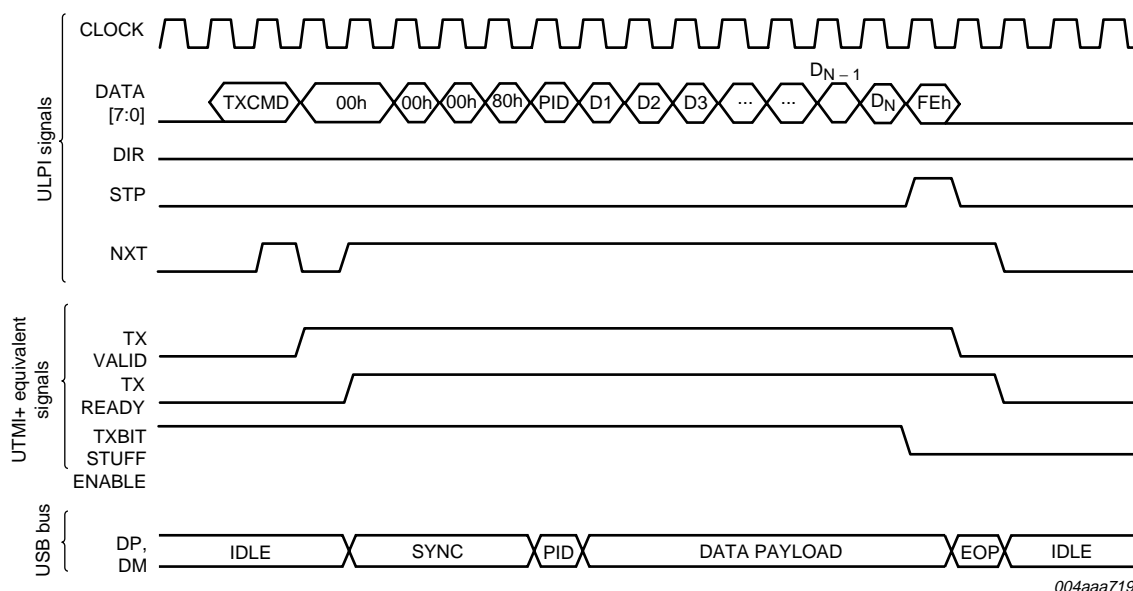
Fig 20. Transmitting USB packets without automatic SYNC and EOP generation
