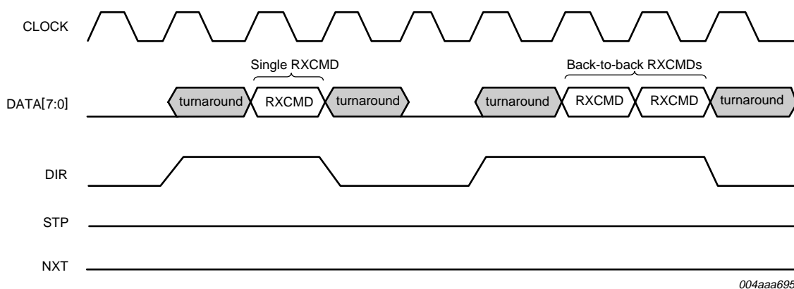
Fig 9. Single and back-to-back RXCMDs from the ISP1504x1 to the link
