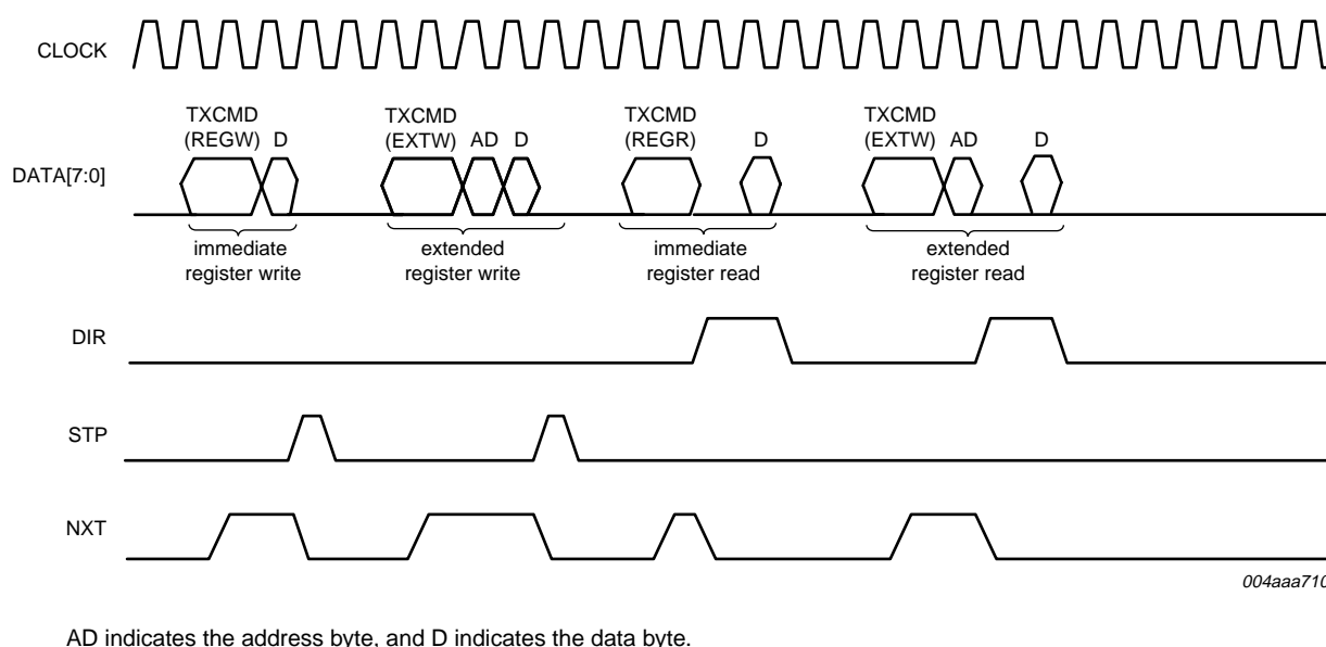
Fig 11. Example of register write, register read, extended register write and extended register read
