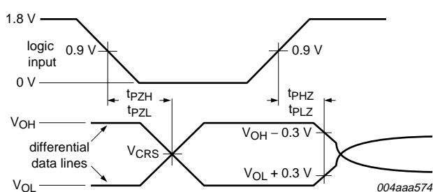
Fig 28. Timing of TX_ENABLE to DP and DM
