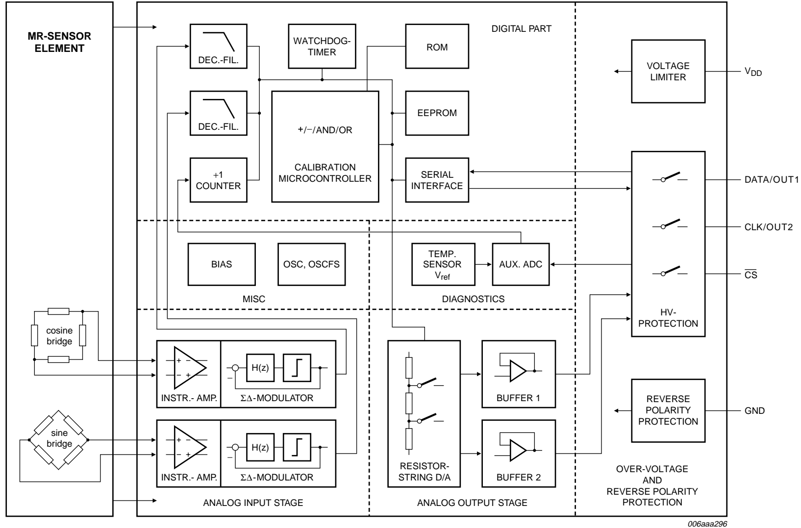
Fig 1. Functional diagram
