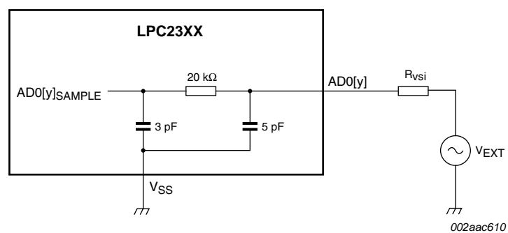
Fig 15. Suggested ADC interface - LPC2364/65/66/67/68 AD0[y] pin
