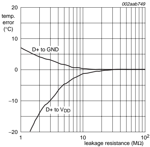
Fig 6. Temperature error versus printed-circuit board leakage resistance
