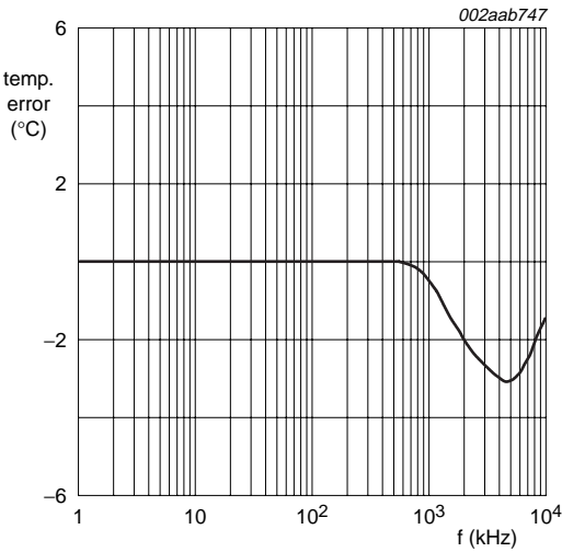
Fig 7. Temperature error versus common-mode noise frequency
