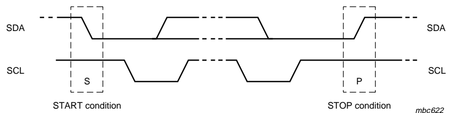
Fig 28. Definition of START and STOP conditions
