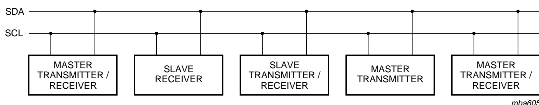
Fig 11. System configuration
