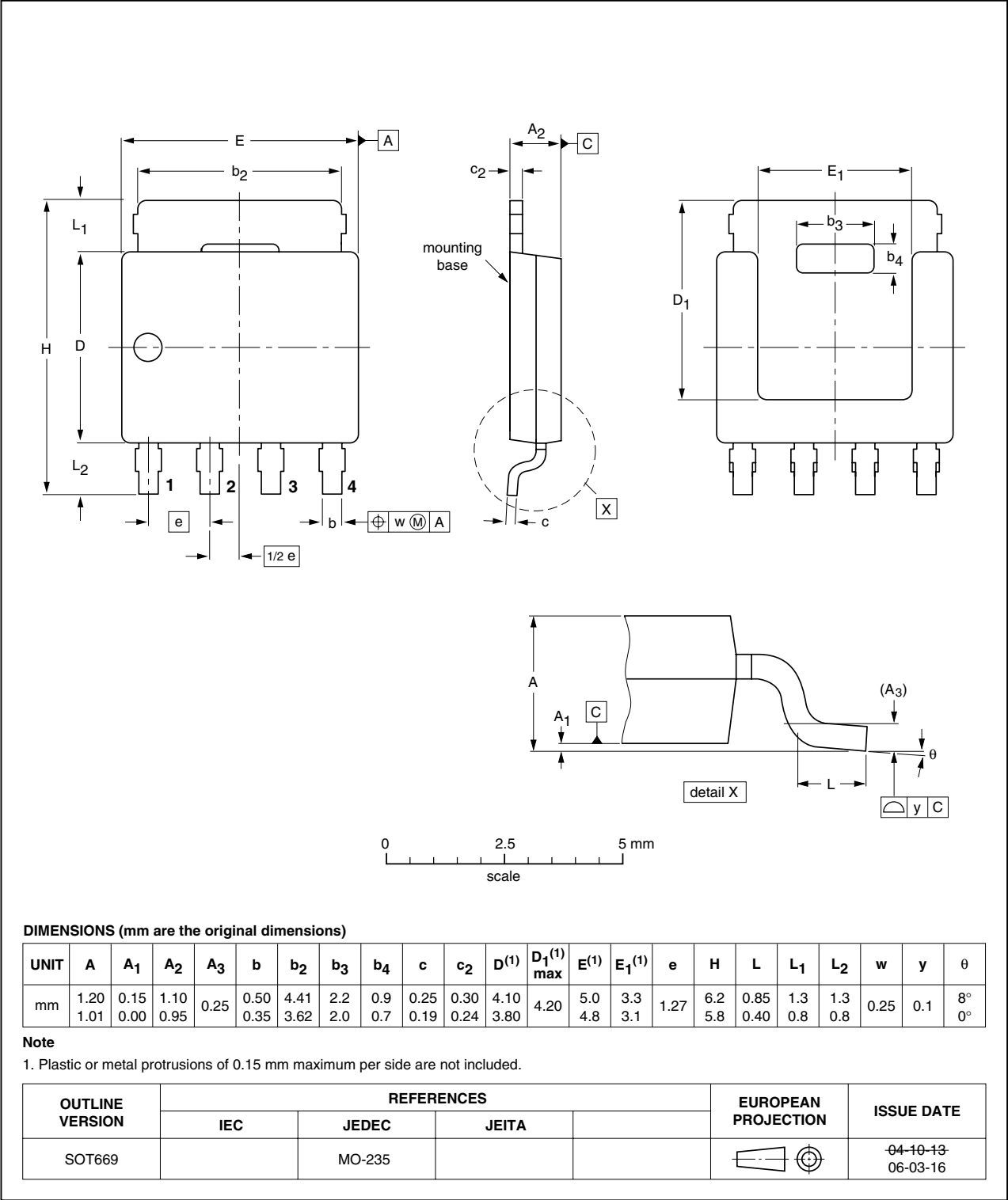
Fig 13. Package outline SOT669 (LFAK)
