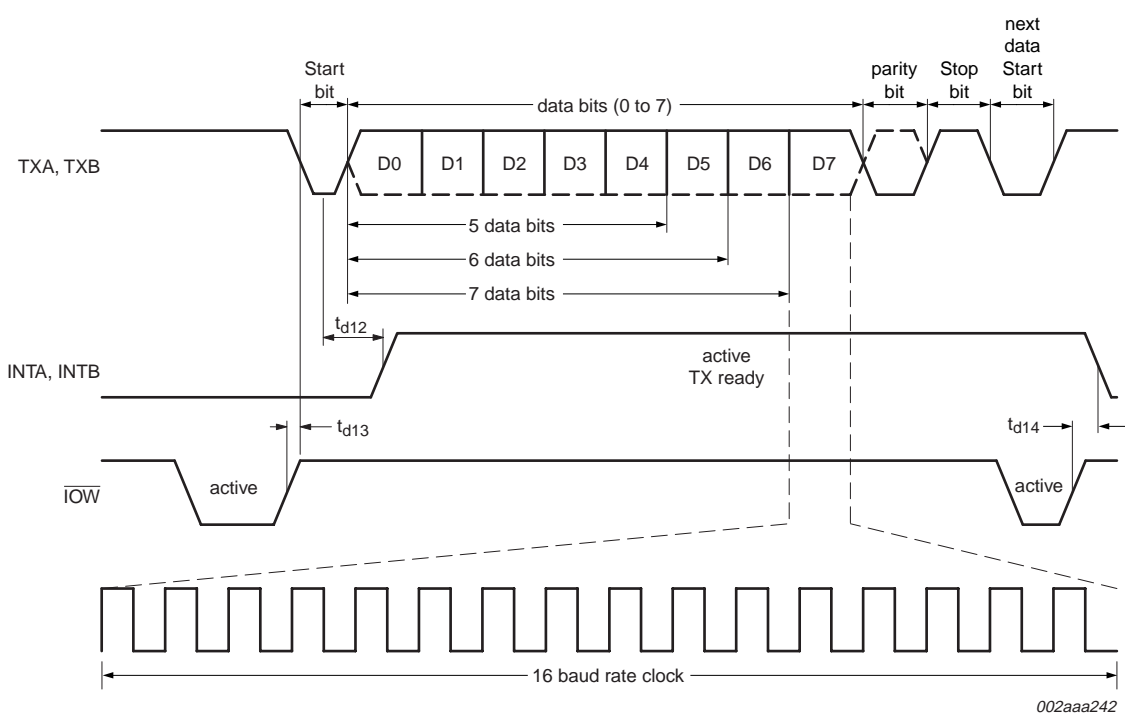
Fig 20. Transmit timing
