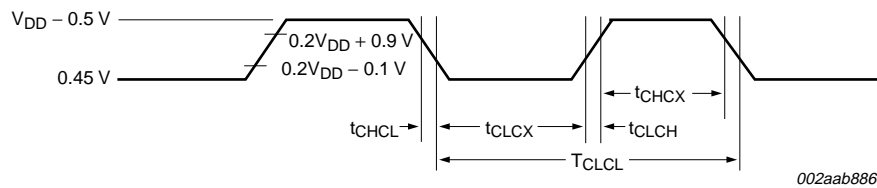
Fig 23. External clock timing
