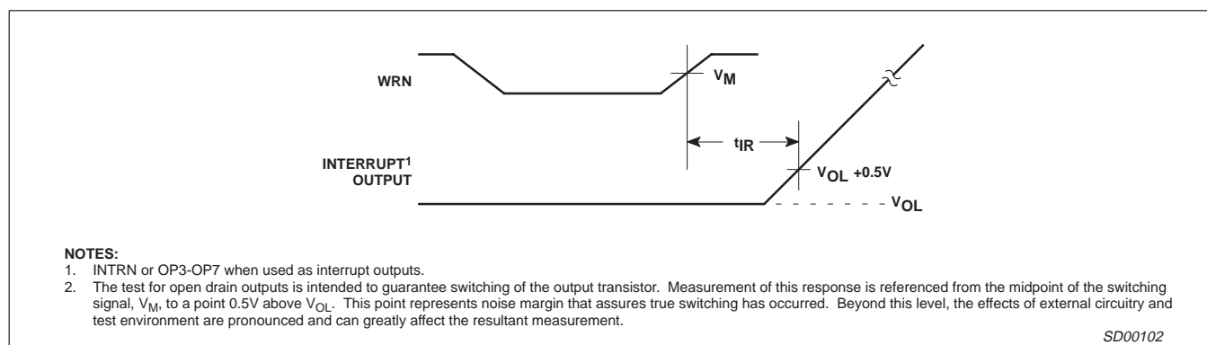
Figure 6. Interrupt Timing
