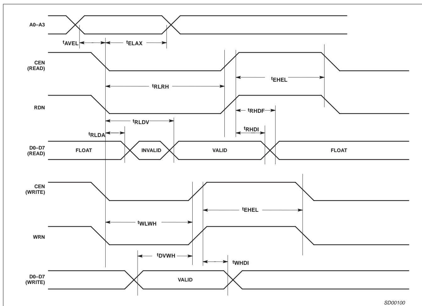
Figure 4. Bus Timing
