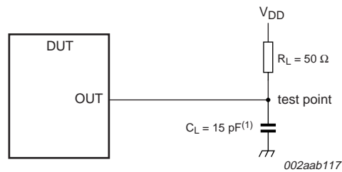
Fig 12. Load circuit, HIGH-to-LOW slew measurement
