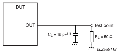
Fig 14. Load circuit, LOW-to-HIGH slew measurement
