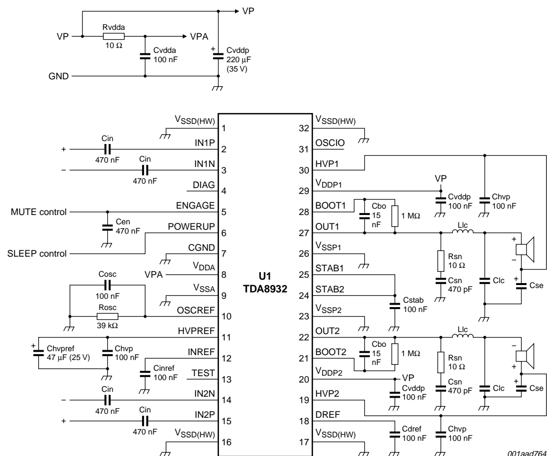
Fig 28. Typical simplified application diagram for 2 × SE (asymmetrical supply)
