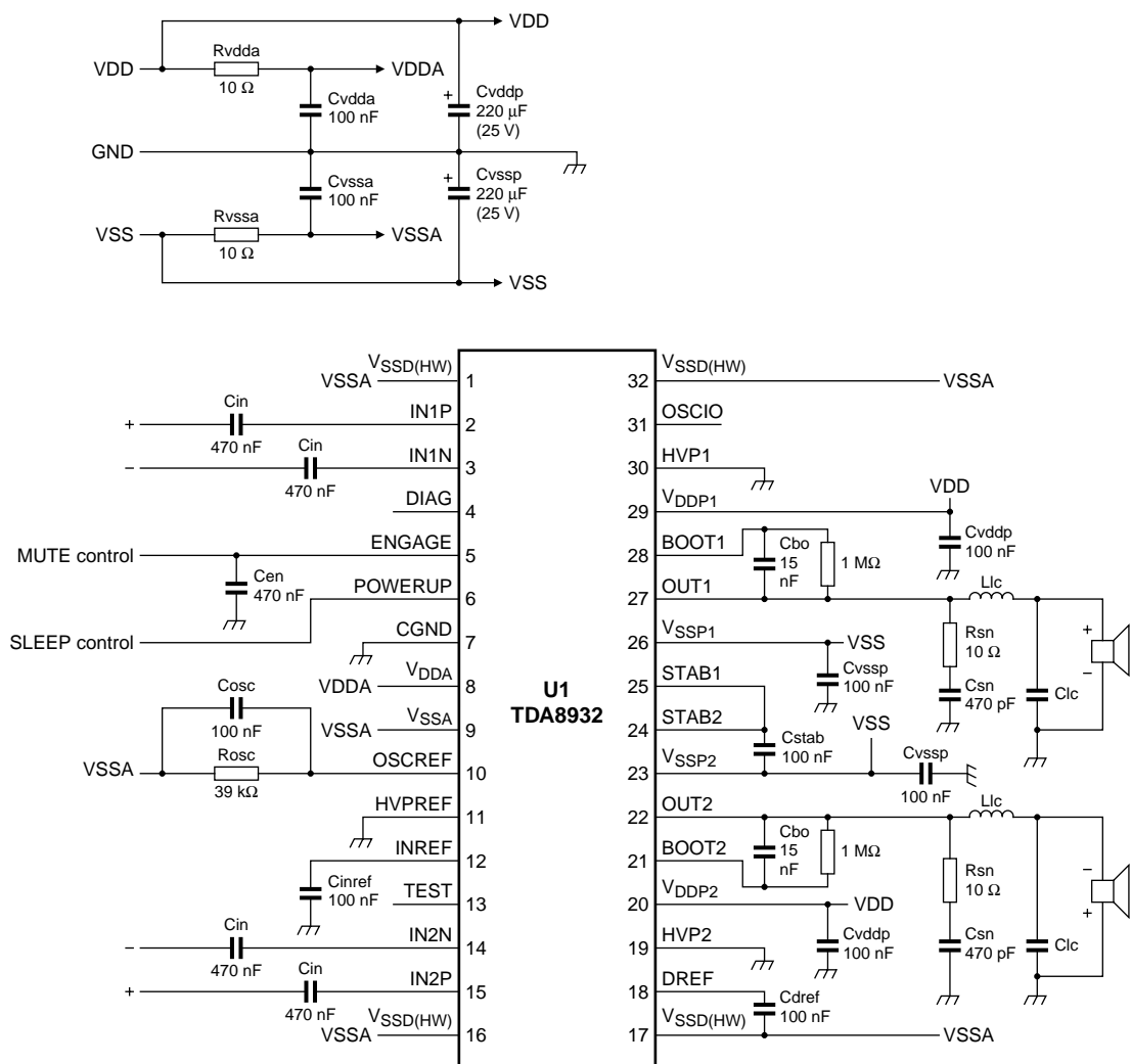
Fig 30. Typical simplified application diagram for 2 x SE (symmetrical supply)
