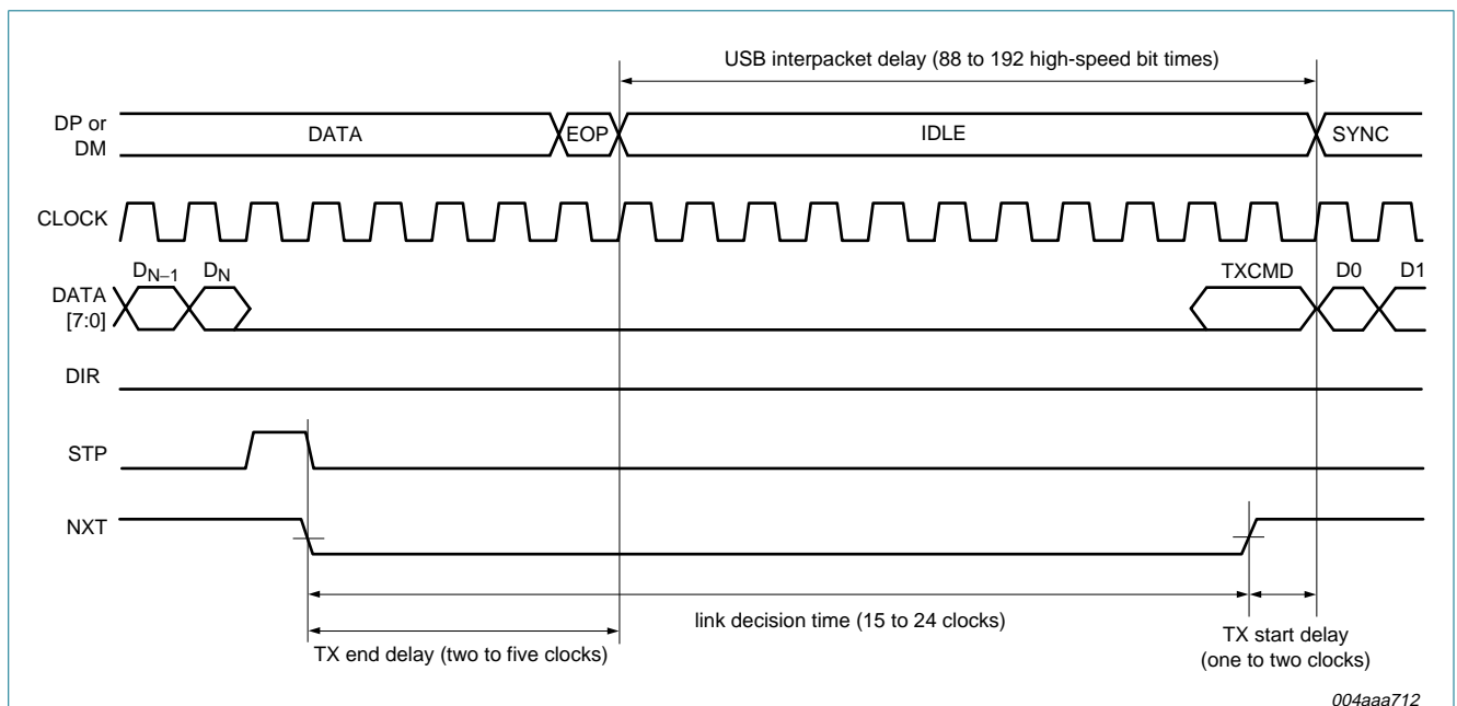
Fig 11. High-speed transmit-to-transmit packet timing
