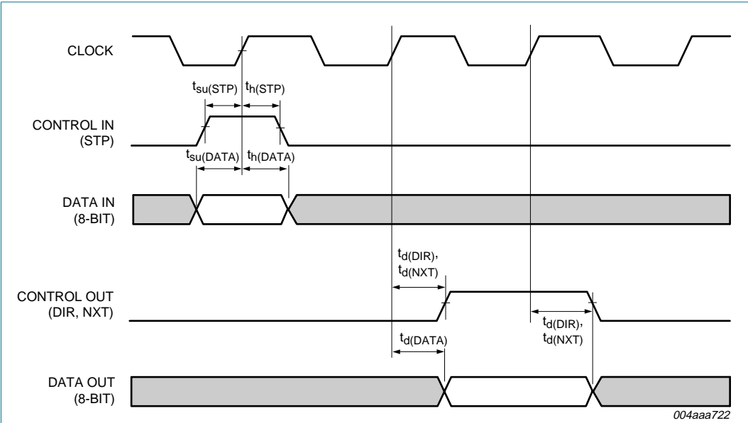
Fig 25. ULPI timing interface
