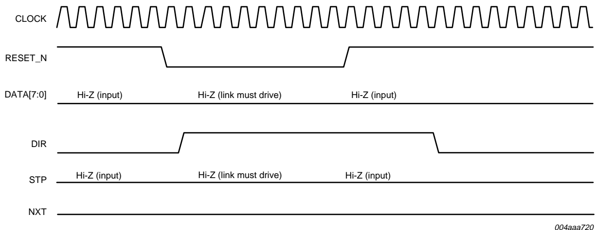
Fig 5. Interface behavior with respect to RESET_N
