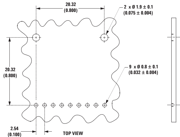
Figure 8. Recommended Board Layout Hole Pattern
