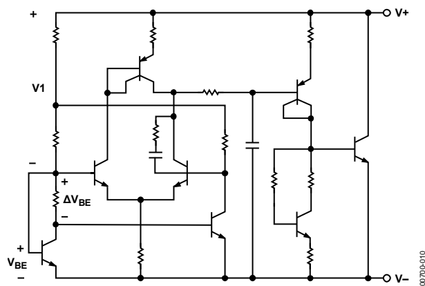
Figure 10. Schematic Diagram
