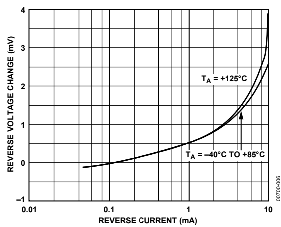
Figure 6. Reverse Voltage Change vs. Reverse Current
