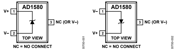
Figure 1. SOT-23
