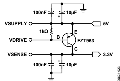
Figure 23. Recommended 3.3 V Regulator Circuit
