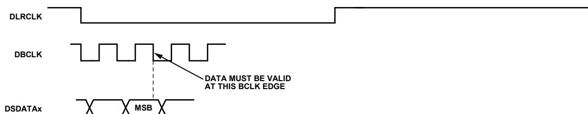
Figure 20. I²S Pipeline Mode in DAC Serial Data Transmission (Applicable in Stereo and TDM Useful for High Frequency TDM Transmission)
