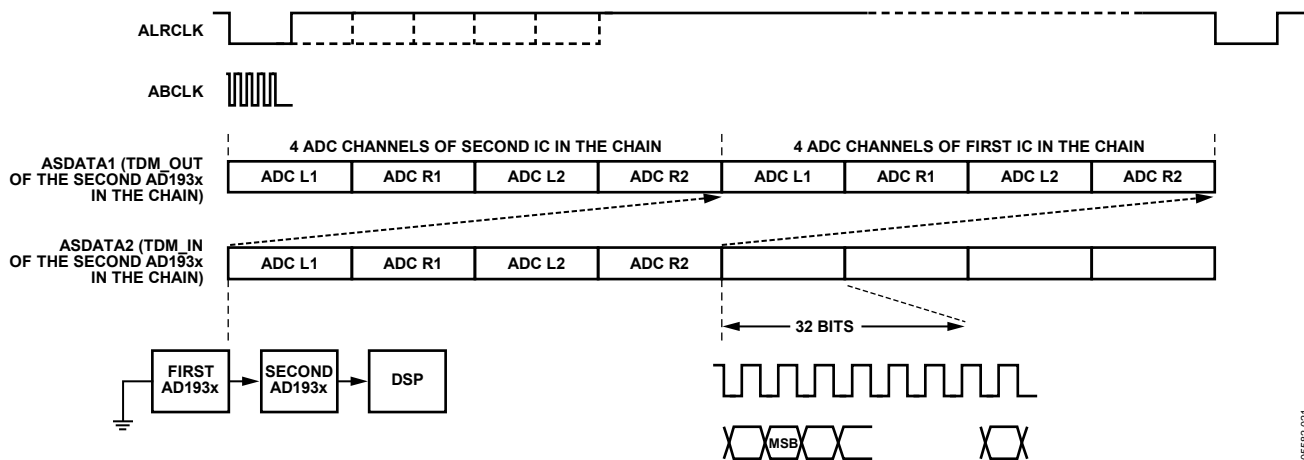
Figure 21. ADC TDM Daisy-Chain Mode (256 fs BCLK, Two-AD1938x Daisy Chain)
