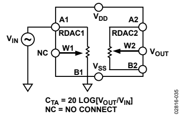
Figure 34. Analog Crosstalk
