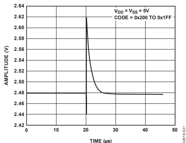
Figure 20. Midscale Glitch Energy, R_{AB} = 25 \text{ k}\Omega , Code 0x200 to Code 0x1FF
