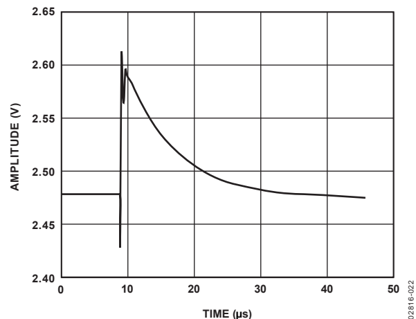
Figure 21. Midscale Glitch Energy, R_{AB} = 250 \text{ k}\Omega , Code 0x200 to Code 0x1FF
