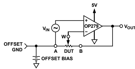
Figure 30. Noninverting Gain
