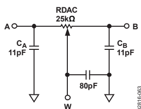
Figure 62. RDAC Circuit Simulation Model (RDAC = 25 k \Omega )
