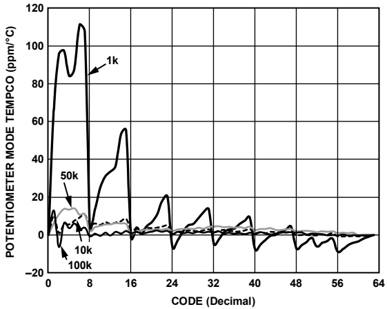
Figure 18. Potentiometer Mode Tempco ( \Delta V_W \times 10^6 / (V_W \times \Delta T) ) vs. Code
