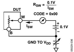
Figure 35. Test Circuit for Common-Mode Leakage Current
