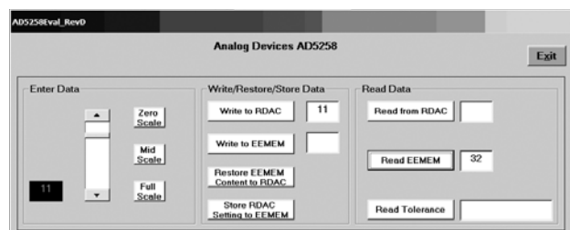
Figure 43. AD5258 Evaluation Board Software
