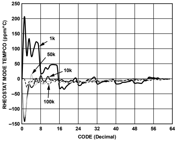
Figure 17. Rheostat Mode Tempco ( \Delta R_{AB} \times 10^6 / (R_{AB} \times \Delta T) ) vs. Code
