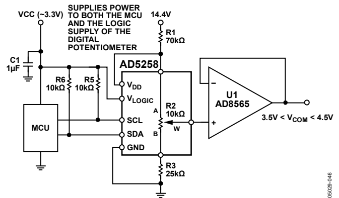
Figure 45. Circuitry When a Separate Supply Is Not Available for V_{\text{DD}}
