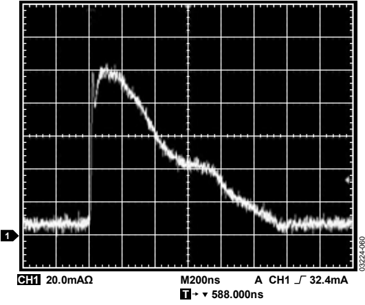
Figure 28. OTP Program Energy Plot for Single Fuse
