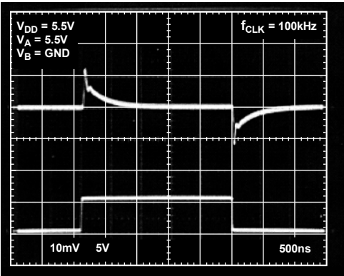
Figure 23. Digital Feedthrough
