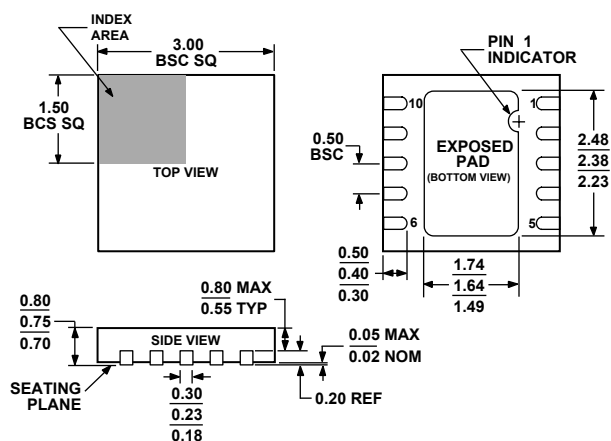
Figure 46. 10-Lead Lead Frame Chip Scale Package [LFCSP_WD] 3 mm x 3 mm Body, Very Very Thin, Dual Lead (CP-10-9)
