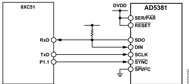
Figure 37. AD5381-to-8051 Interface
