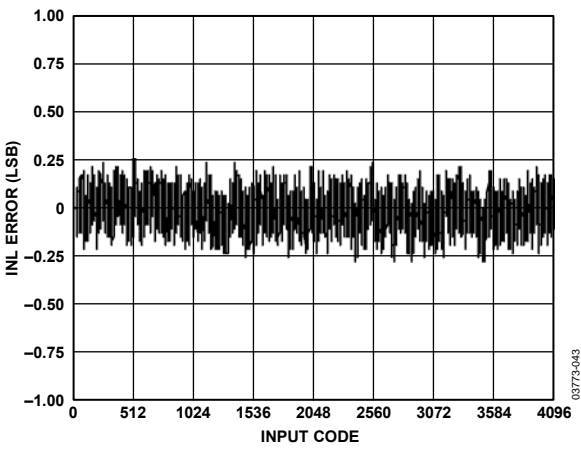
Figure 14. Typical AD5391-5 INL Plot
