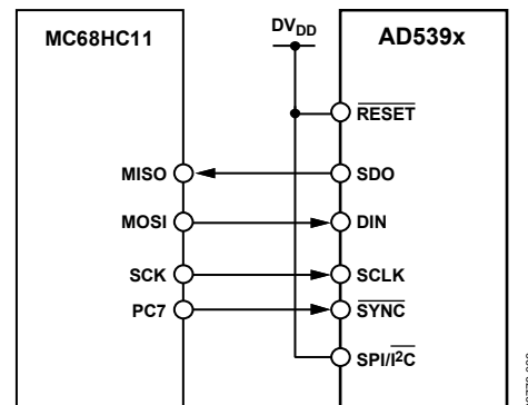
Figure 37. AD539x-MC68HC11 Interface
