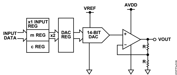
Figure 31. Single-Channel Architecture
