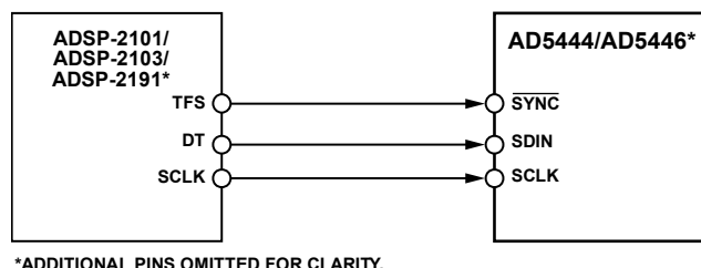
Figure 47. ADSP-2101/ADSP-2103/ADSP-2191 SPORT to AD5444/AD5446 Interface
