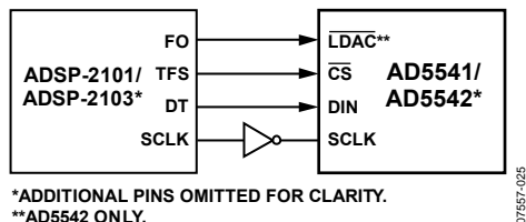
Figure 25. AD5541/AD5542 to ADSP-2101/ADSP-2103 Interface
