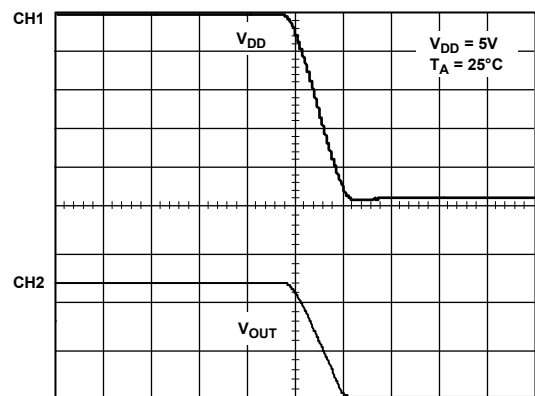
Figure 17. V_{DD} vs. V_{OUT}
