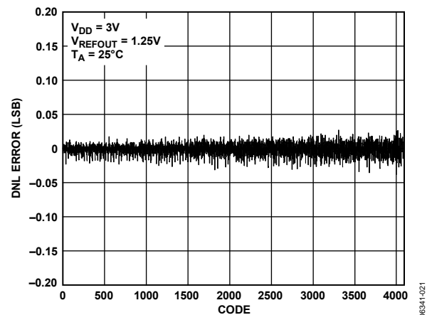
Figure 25. DNL, AD5625R, 1.25 V Internal Reference
