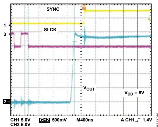
Figure 41. Exiting Power-Down to Midscale
