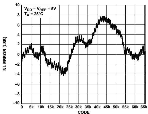
Figure 6. AD5667 INL, External Reference
