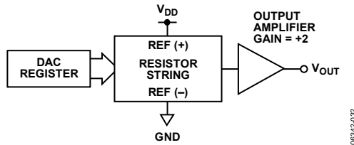
Figure 52. DAC Architecture
