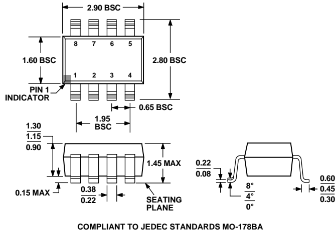
Figure 45. 8-Lead SOT-23 (RJ-8) Dimensions shown in millimeters
