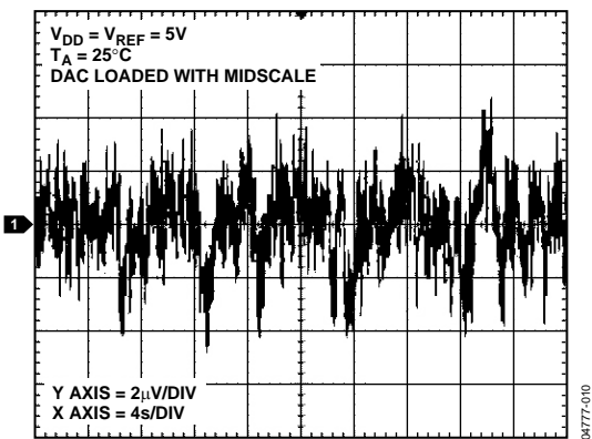
Figure 30. 0.1 Hz to 10 Hz Output Noise Plot
