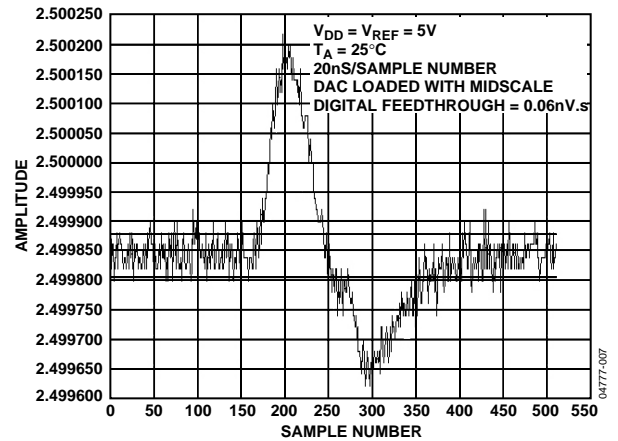
Figure 27. Digital Feedthrough
