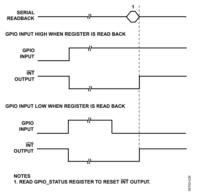
Figure 42. INT Output Controlled by the GPIO Input Example, GPIO_SETUP = 01, GPIO_INPUT_CONFIG = 01
