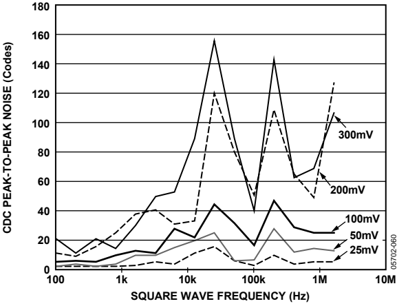
Figure 17. Power Supply Square Wave Rejection
