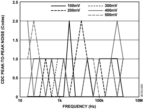
Figure 16. Power Supply Sine Wave Rejection
