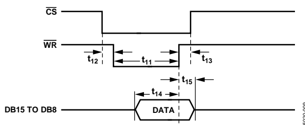
Figure 29. Parallel Interface—Write Cycle for Word Mode ( \overline{\text{W/B}}=0 )
