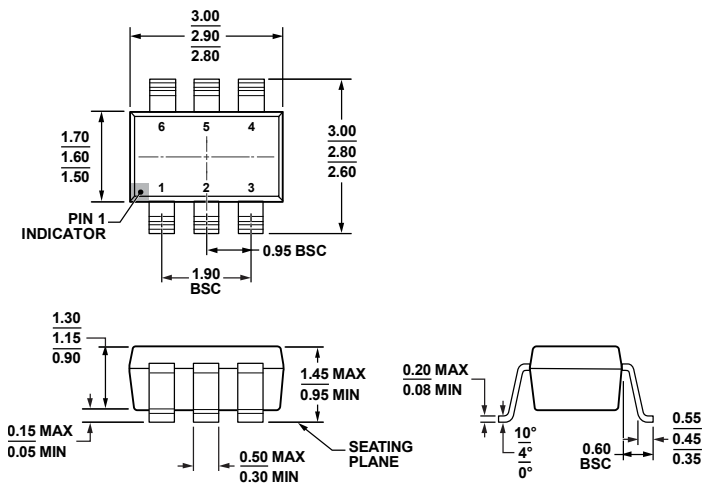
Figure 60. 6-Lead Small Outline Transistor Package [SOT-23] (RJ-6) Dimensions shown in millimeters
