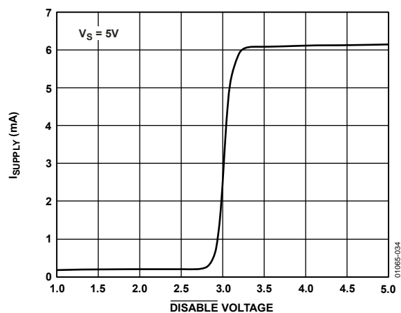
Figure 34. AD8063 \overline{\text{DISABLE}} Voltage vs. Supply Current
