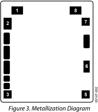
Figure 3. Metallization Diagram
