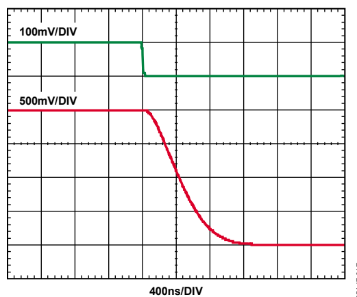
Figure 9. Fall Time
