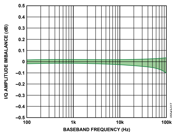
Figure 17. Representative Range of I/Q Amplitude Imbalance vs. Baseband Frequency, Channel 1 and Channel 2 (see Figure 43)
