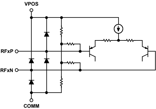
Figure 6. RF Inputs
