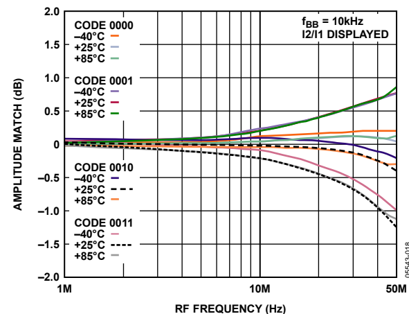
Figure 18. Typical I2xO/I1xO or Q2xO/Q1xO Amplitude Match vs. RF Frequency, First Quadrant, at Three Temperatures
