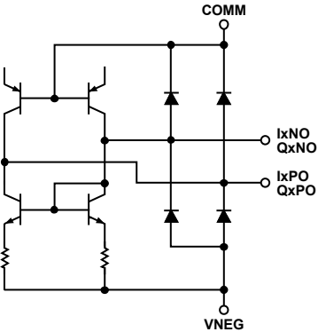
Figure 7. Output Drivers
