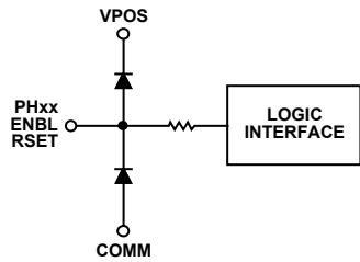
Figure 3. Logic Inputs
