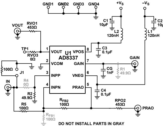
Figure 81. Schematic—AD8337-EVALZ-INV Inverting Configuration
