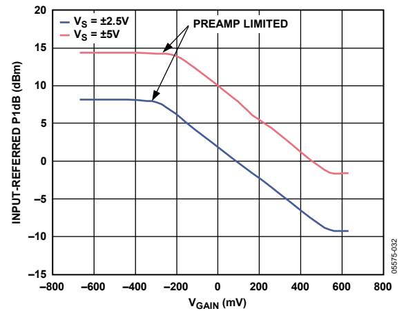
Figure 32. Input-Referred P1dB (IP1dB) vs. V_{GAIN} (See Figure 63)
