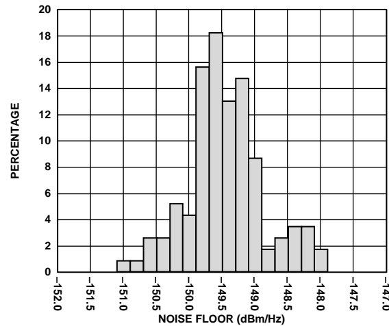
Figure 28. 20 MHz Offset Noise Floor Distribution at F_{LO} = 940 MHz ( F_{BB} = 1 MHz, I and Q Inputs Driven in Quadrature at 1.2 V p-p, T_A = 25^\circ\text{C} )
