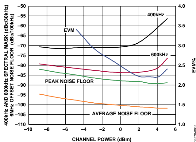
Figure 62. GMSK EVM, Spectral Performance, and Noise Floor vs. Channel Power (Frequency = 885 MHz)
