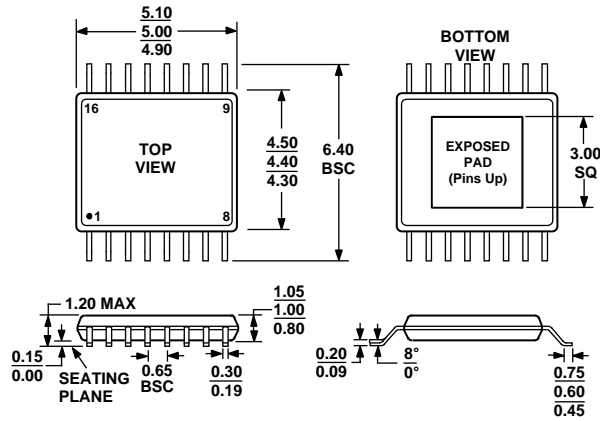
Figure 70. 16-Lead Thin Shrink Small Outline with Exposed Pad [TSSOP/EP] (RE-16-2)
