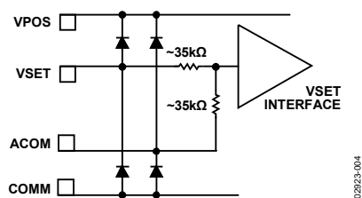
Figure 4. Circuit B
