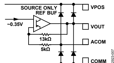
Figure 7. Circuit E
