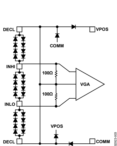
Figure 3. Circuit A
