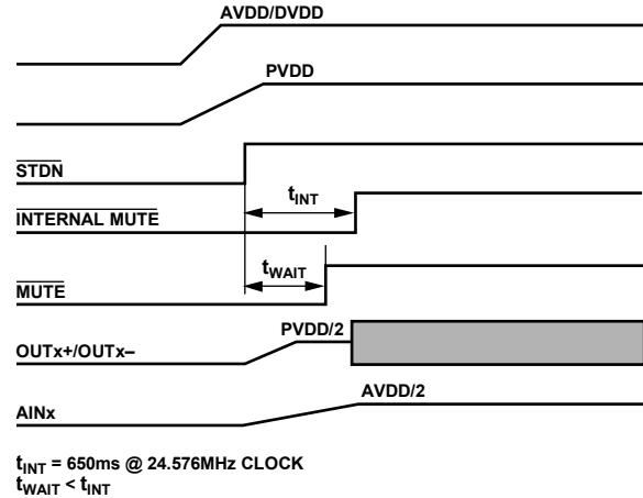
Figure 47. Power-Up Sequence, t_{WAIT} < t_{INT}
