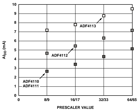
Figure 25. AL_{DD} vs. Prescaler Value
