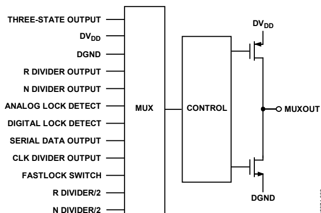
Figure 15. MUXOUT Schematic
