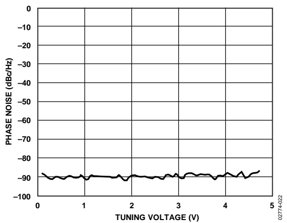
Figure 22. IF Noise vs. V_{TUNE}
