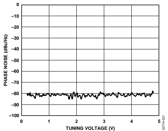
Figure 21. RF Noise vs. V_{TUNE}
