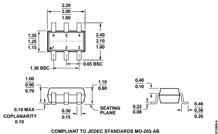
COMPLIANT TO JEDEC STANDARDS MO-203-AB Figure 23. 6-Lead Plastic Surface Mount Package [SC70] (KS-6) Dimensions shown in millimeters
