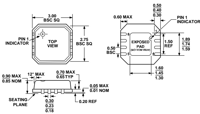
Figure 19. 8-Lead Lead Frame Chip Scale Package [LFCSP_VD] 3 mm × 3 mm Body, Very Thin, Dual Lead (CP-8-2) Dimensions shown in millimeters
