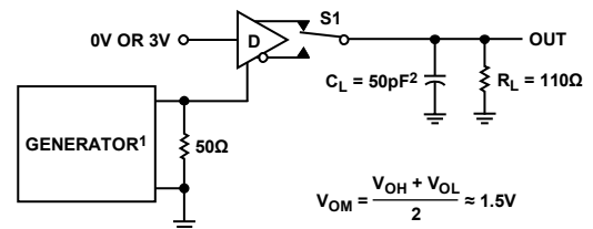
Figure 7. Driver Propagation Delays
