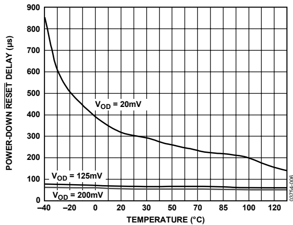
Figure 7. Power-Down \overline{\text{RESET}} Delay vs. Temperature: ADM671_L/M
