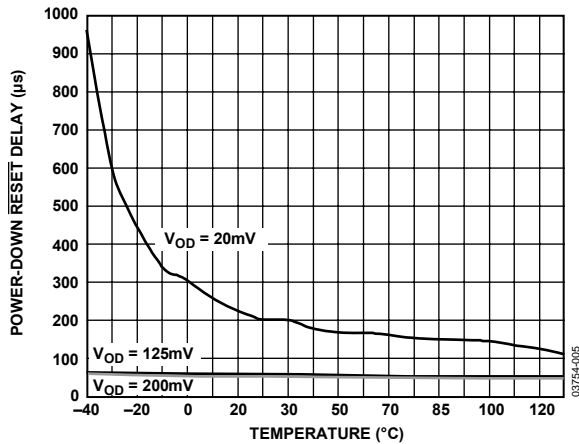
Figure 6. Power-Down \overline{\text{RESET}} Delay vs. Temperature: ADM671_R/S/T/Z
